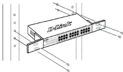
Figure 3. Installing the switch in a standard-sized equipment rack
