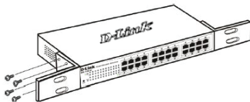
Figure 2. Attaching the mounting brackets
