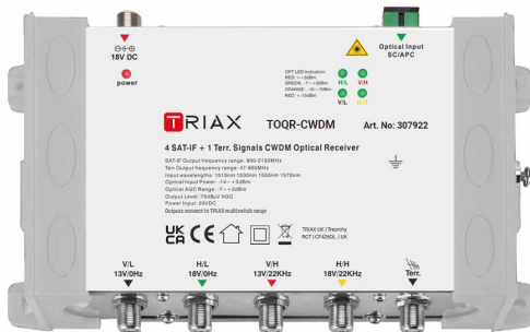
TOQR-CWDM TRIAX Optical Quattro Receiver 4SAT-IF + 1Terr. Signal CWDM Optical Receiver
