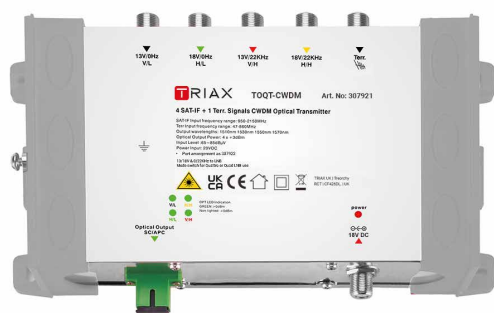
TOQT-CWDM TRIAX Optical Quattro/Quad Transmitter 4SAT-IF + 1Terr. Signal CWDM Optical Transmitter
