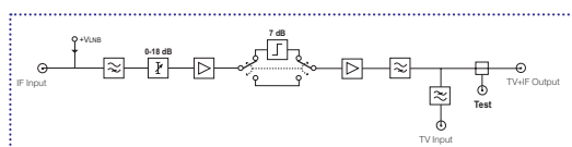
Block Diagram
