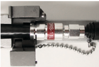
PCT-DRS-11L connector / RG11 coaxial cable
