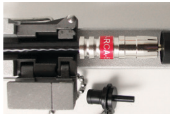
PCT-RCA-59 connector / RG59 coaxial cable
